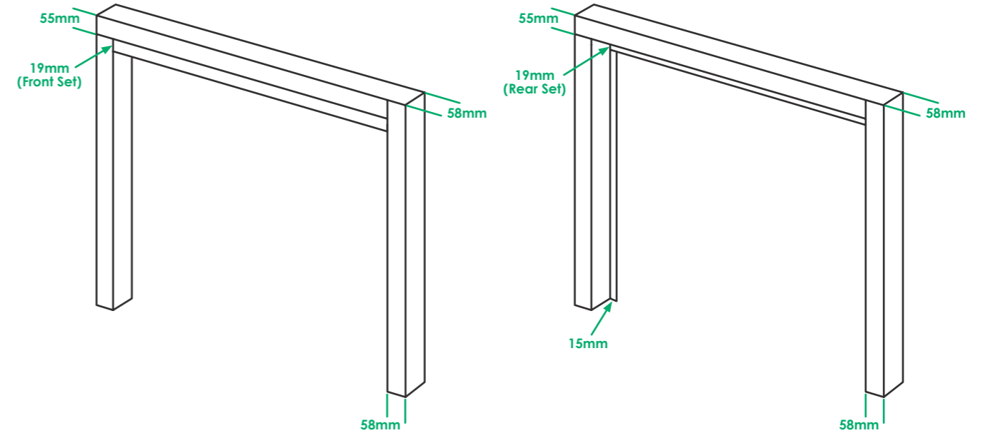
Canopy/Retract Frame
