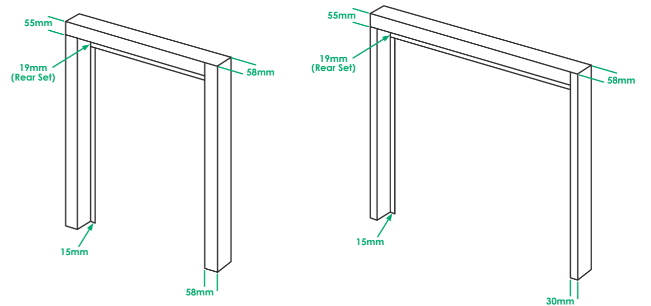
Personnel Frame
